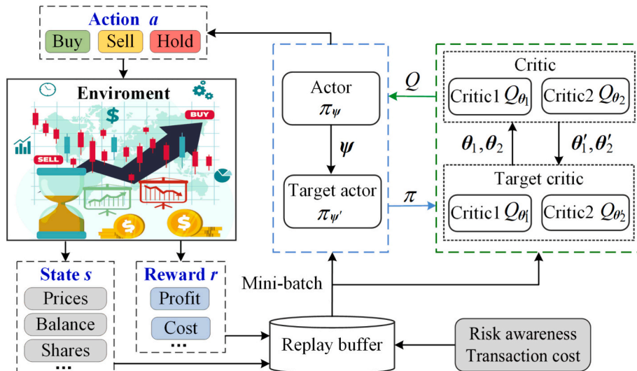
Fig. 1. TD3-based portfolio trading framework.
